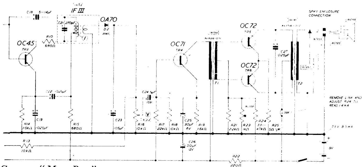
GRUNDIG "MICROBOY"
